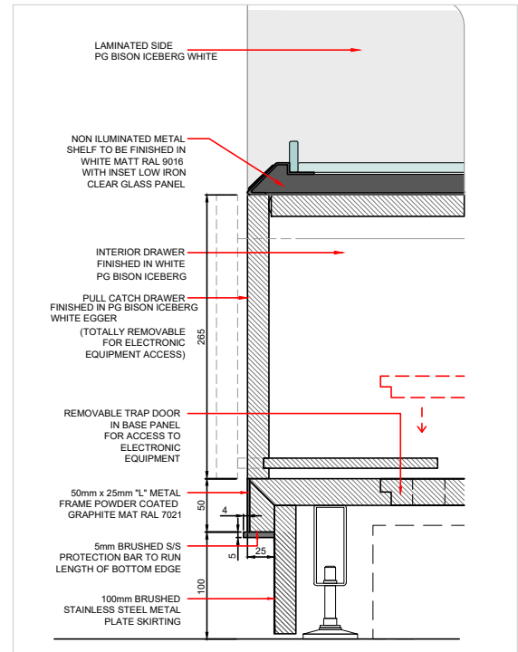
7 BASE DETAIL
